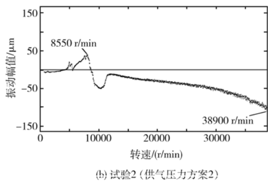
图3 不同轴承供气方案下升速试验分岔图(涡轮端) Fig. 3 Bifurcation plot in raising speed process under different bearing supply pressures (turbine end)
